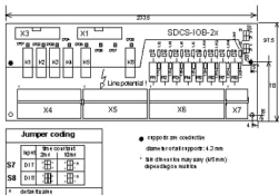
Figure A1.58 Jumper coding of the SDCS-IOB-2x board
